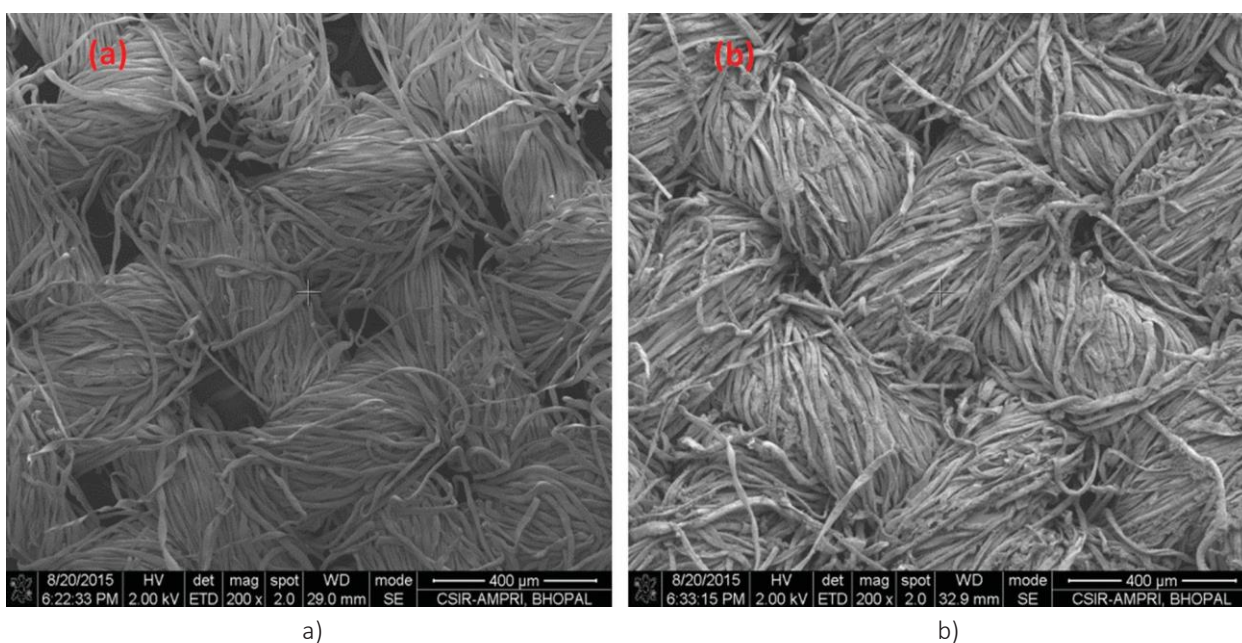
Figure 7. (a) Uncoated cotton fabric (b) MWCNT-coated cotton fabric
