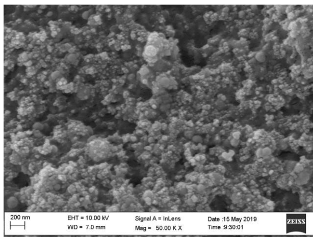
Figure 3. SEM image of PVA film with \text{SiO}_2
