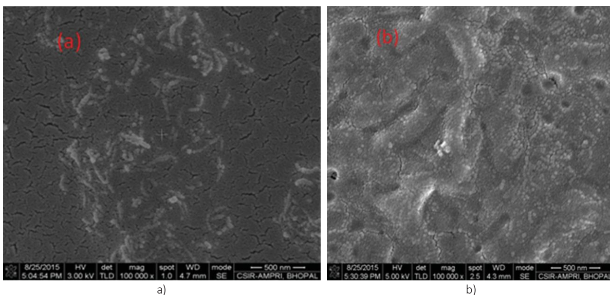
Figure 6. (a) SEM image of untreated MWCNT and (b) SEM image of MWCNT treated with SDS
